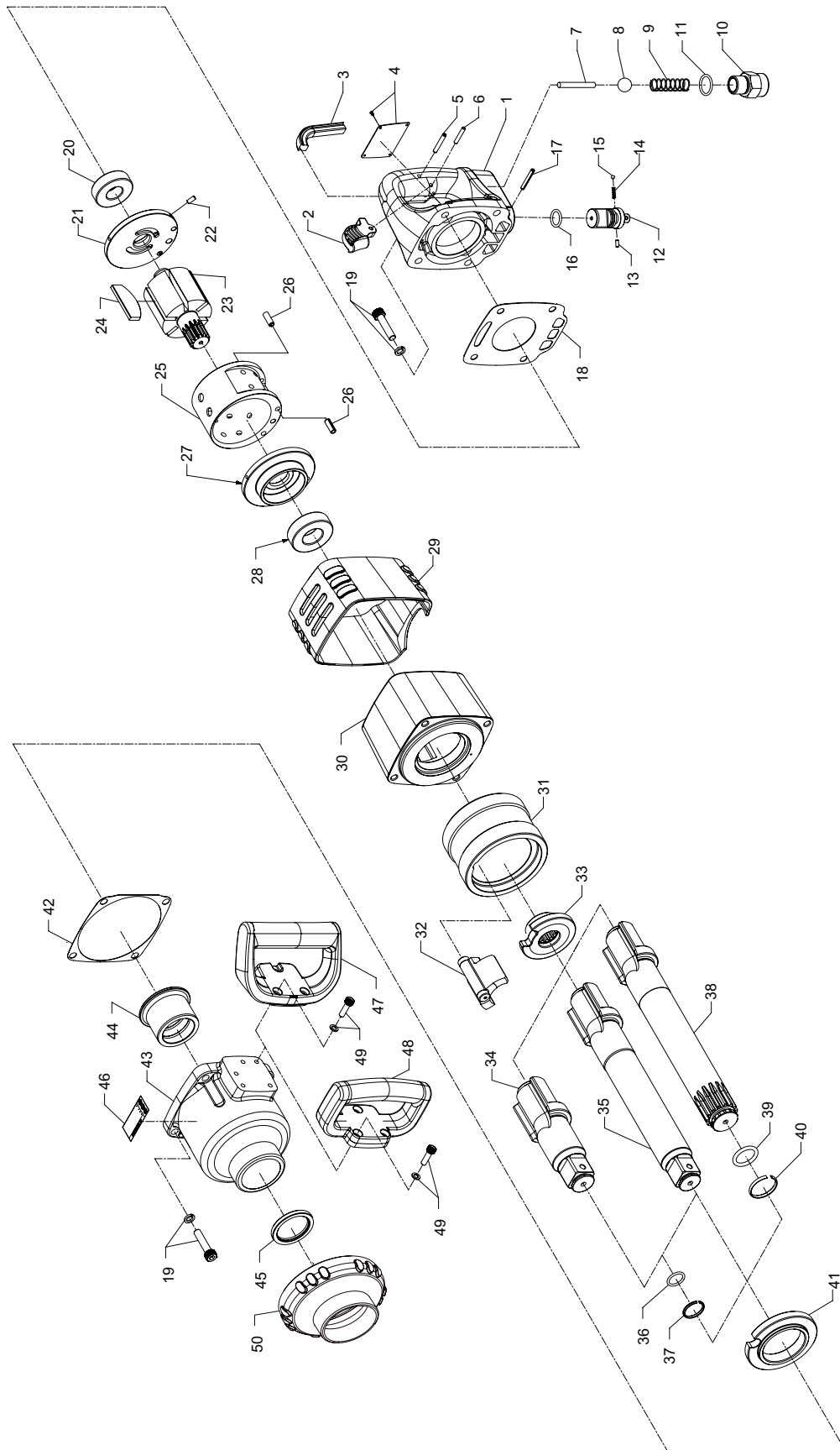
Figure 1. Exploded View - 16578726
